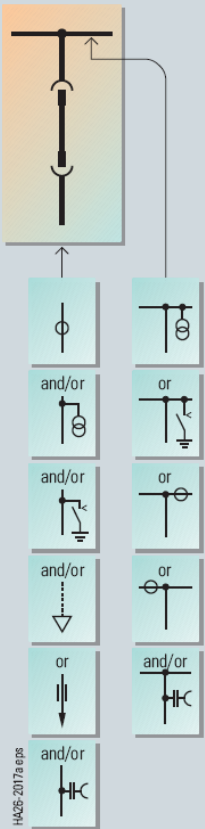
Disconnecting panel
