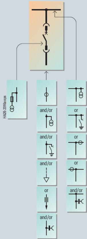
Circuit-breaker panel
