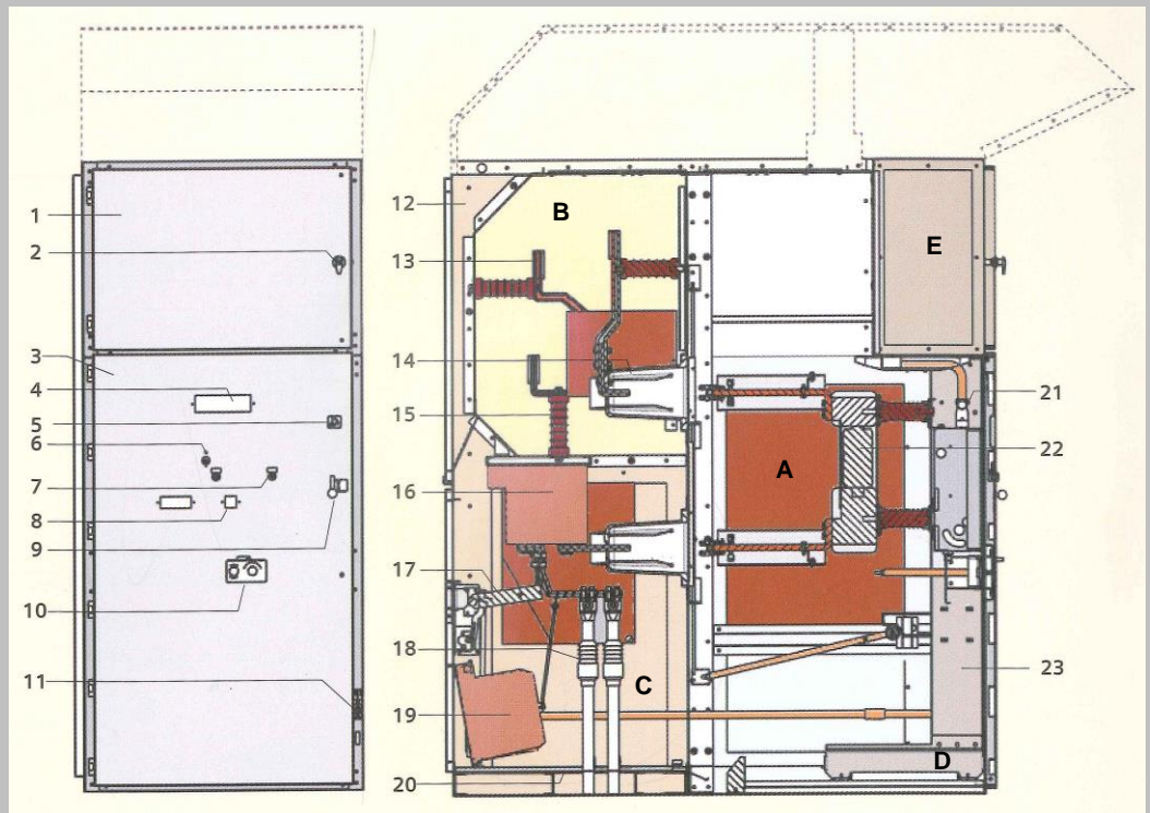
Circuit-breaker panel
